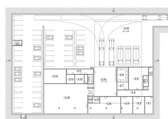
-2nd floor SC 1: 500
