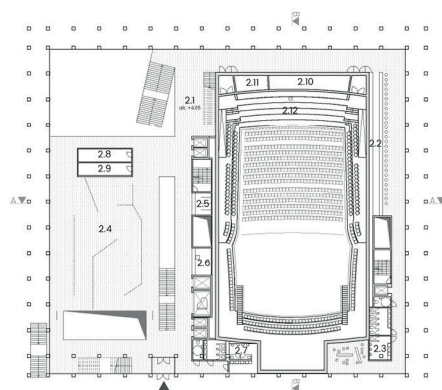
2nd floor SC 1: 500
