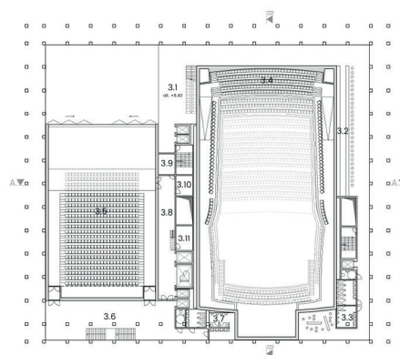
3rd floor SC 1: 500
