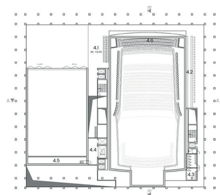
4th floor SC 1: 500
