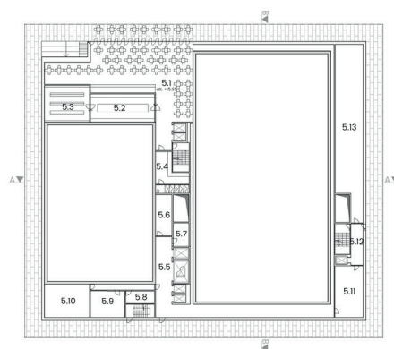
5th floor SC 1: 500
