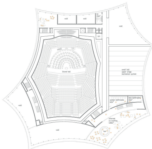
FOURTH FLOOR PLAN scale 1500
