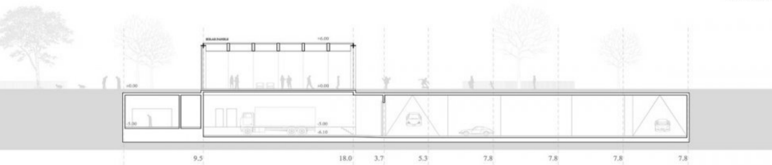
SECTION
