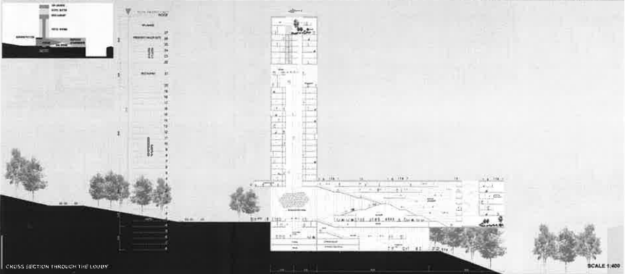
CROSS SECTION THROUGH THE LOBBY
